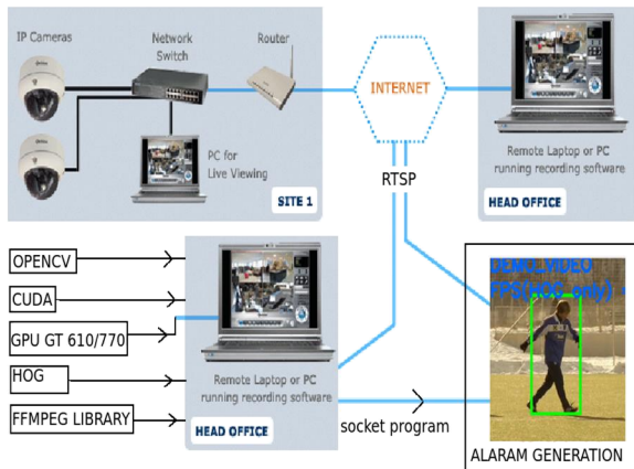
Fig. 4. Block Diagram of the proposed system
