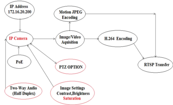
Fig. 5. IP Camera at Server End
