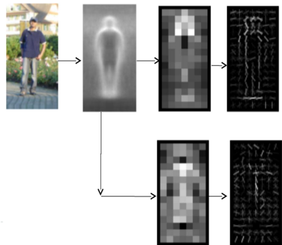
Fig. 3. Results after HOG algorithm for human in standing position.
