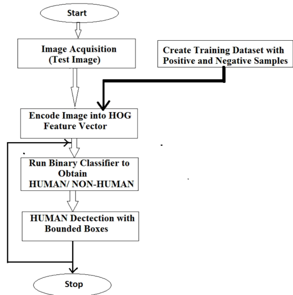
Flowchart. 1. Flow chart for the HOG algorithm
