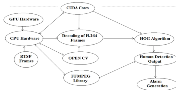
Fig. 7. CPU and GPU at Client End
